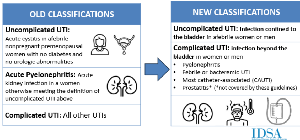
Figure 1: Comparing prior and updated classifications of uncomplicated and complicated UTI
